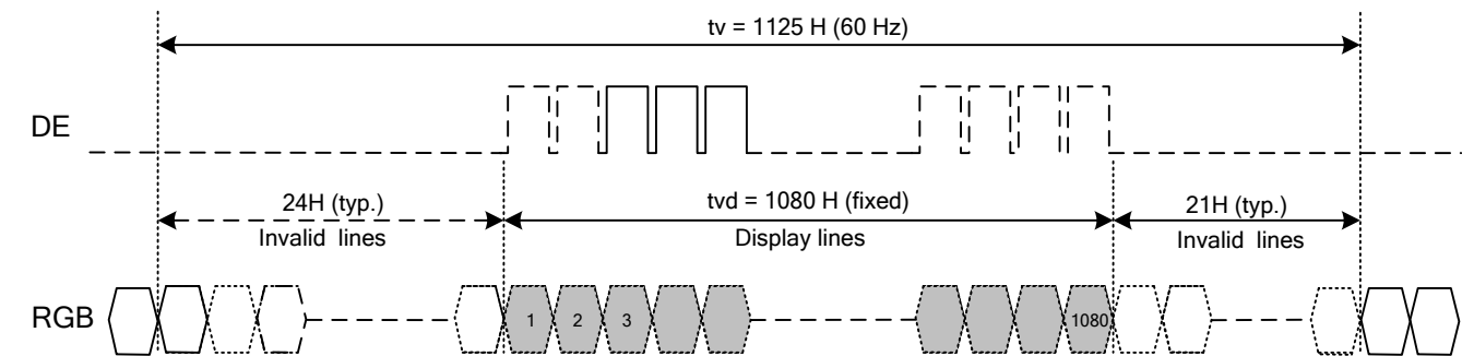
Fig. 9.2 Vertical Timing
