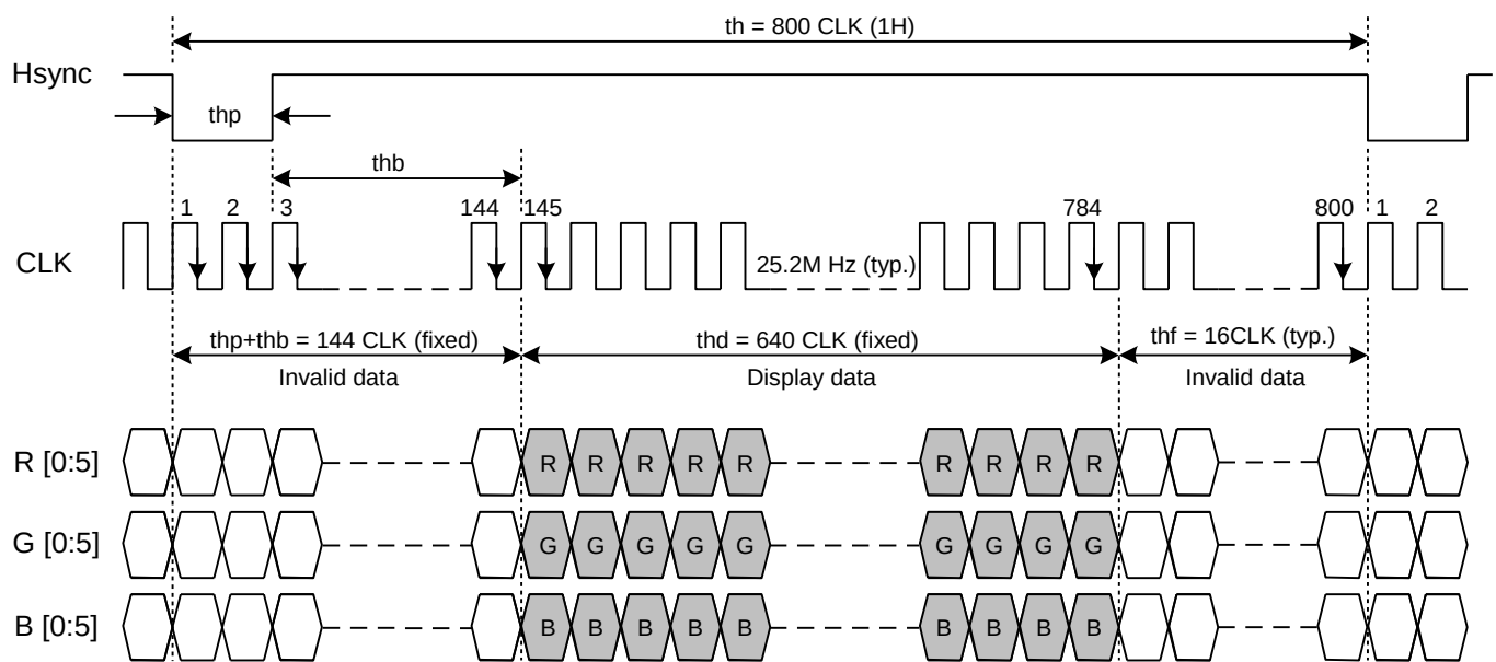
Fig. 9.1 Horizontal Timing
