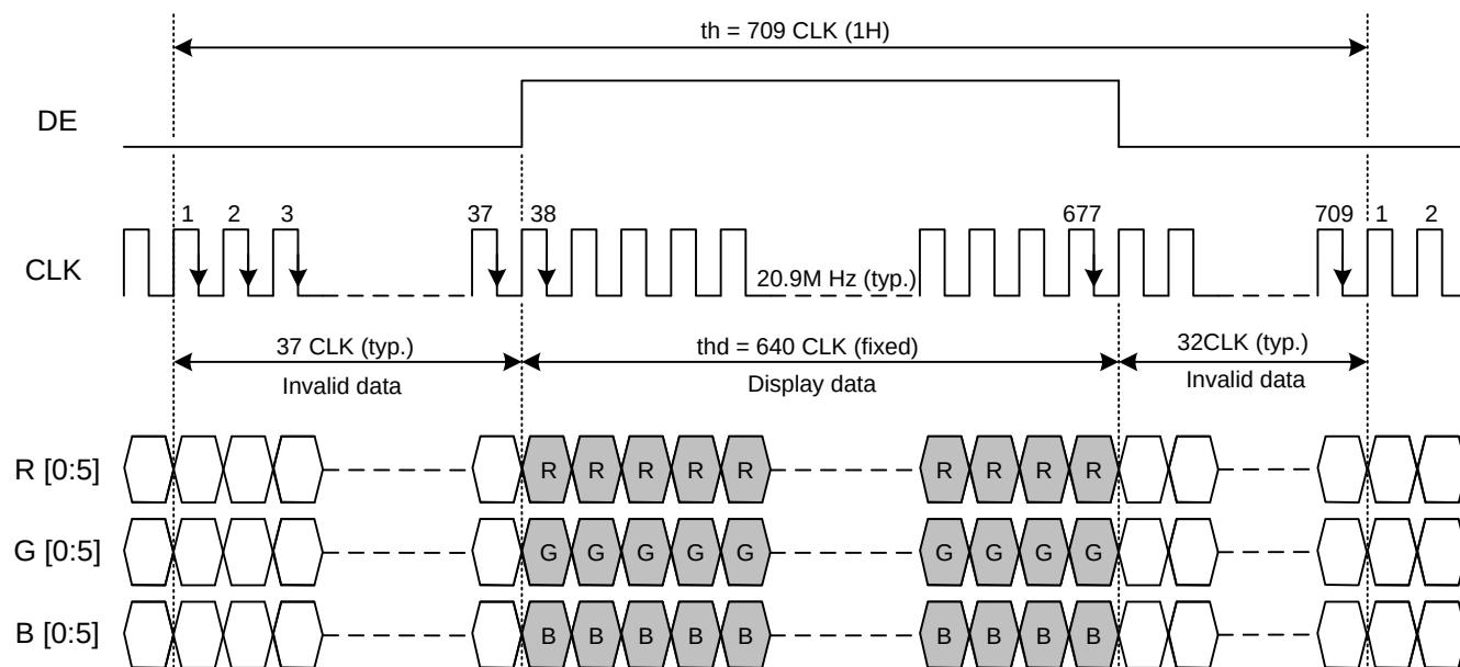
Fig. 9.3 Horizontal Timing
